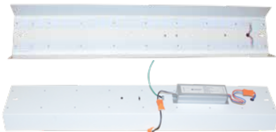
LED RETROFIT LIGHTS FOR EXHAUST CANOPY HOODS
